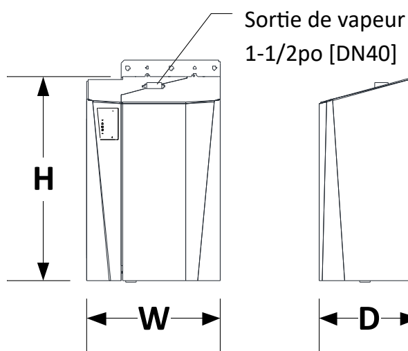
Figure 3 – Dimensions
